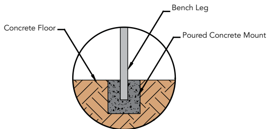
PM - Post Mount Option
