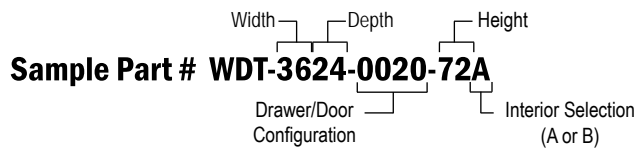
Cabinet Height 72"
