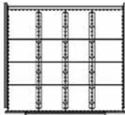
DIV-16_3F12S 16 COMPARTMENT
